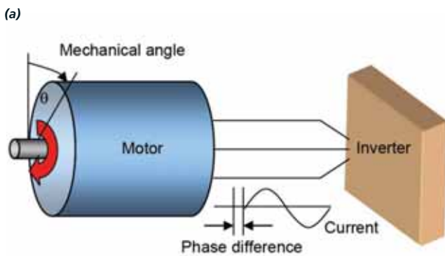
Figure 5: (a) Set-up for measuring electrical angle (b) Screen display of electrical angle measurements
