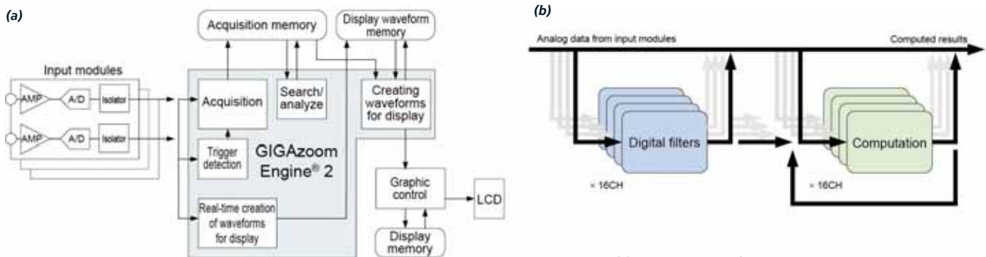
Figure 2: (a) Block diagram of the Yokogawa DL850 ScopeCorder (b) Structure of real-time mathematics unit
