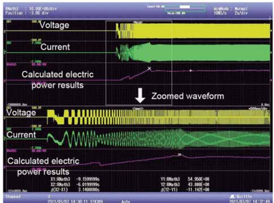
Figure 4: Example of measuring start-up of a motor
